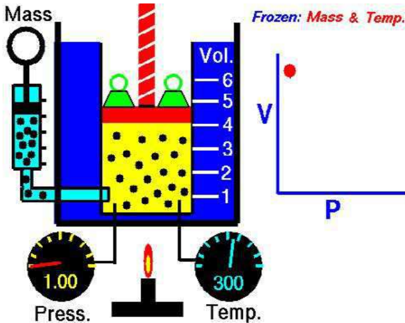
Animation 3.1: Boyle's Law Source & credit: wikipedia
