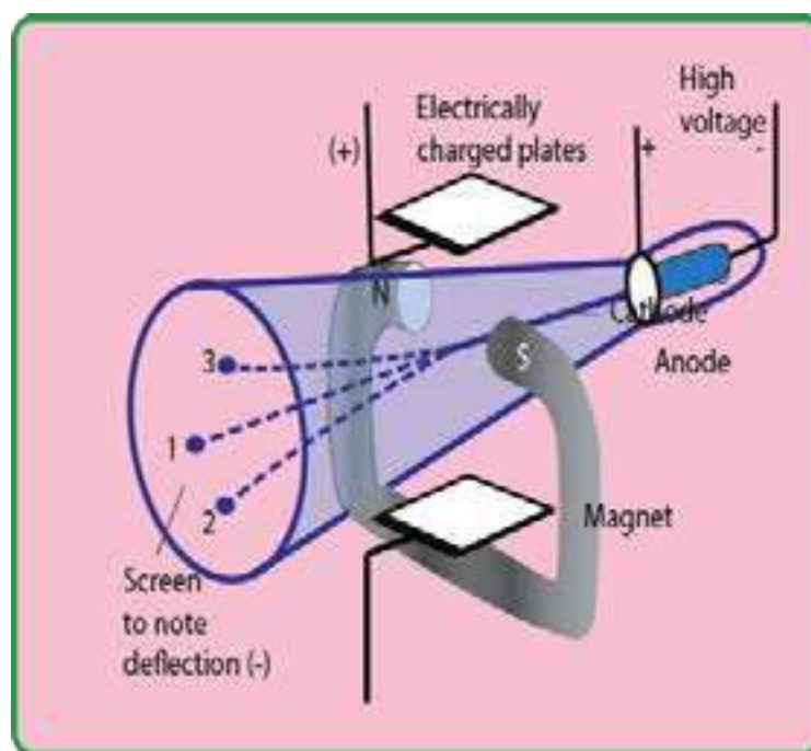
Fig (5.2) Deflection of cathode rays in electric and magnetic fields
