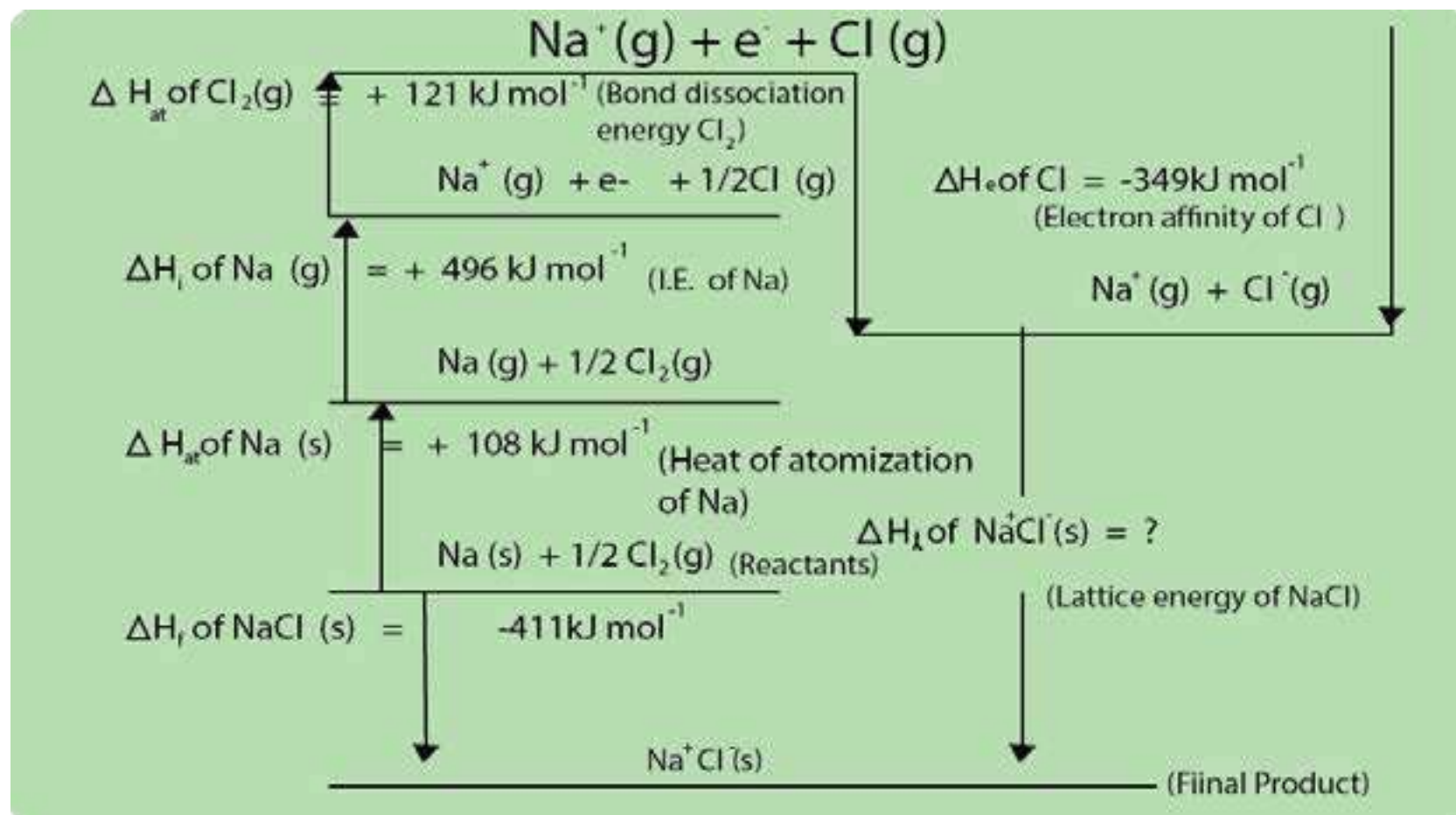
Fig (7.9) Born-Haber cycle
