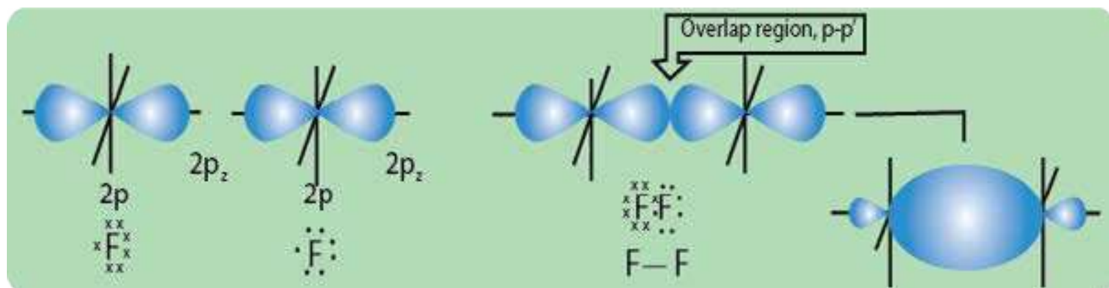
Fig.(6.6) The formation of the fluorine molecule.
