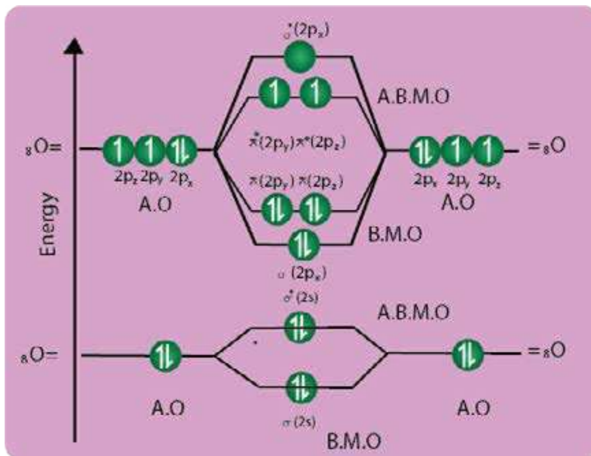
Fig. (6.25) Molecular orbitals in O_2 molecule.
