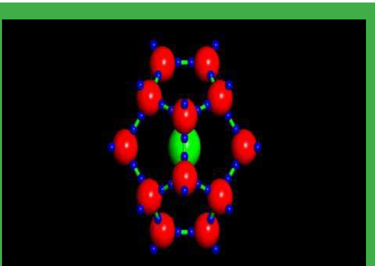
Animation 6.2: Chemical Bond Source & Credit : geo.arizona
