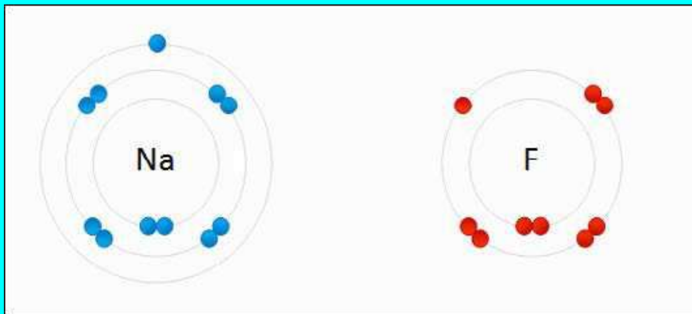
Animation 8.12: COMMON ION Source & Credit : boundless
