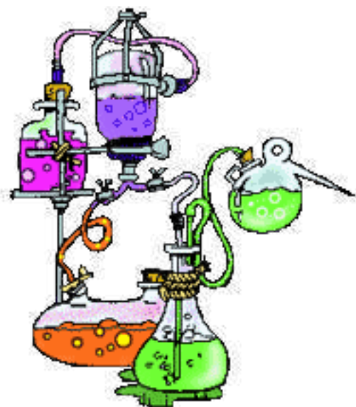
Animation 1.5: Basic Concepts Source & Credit: pixshark
