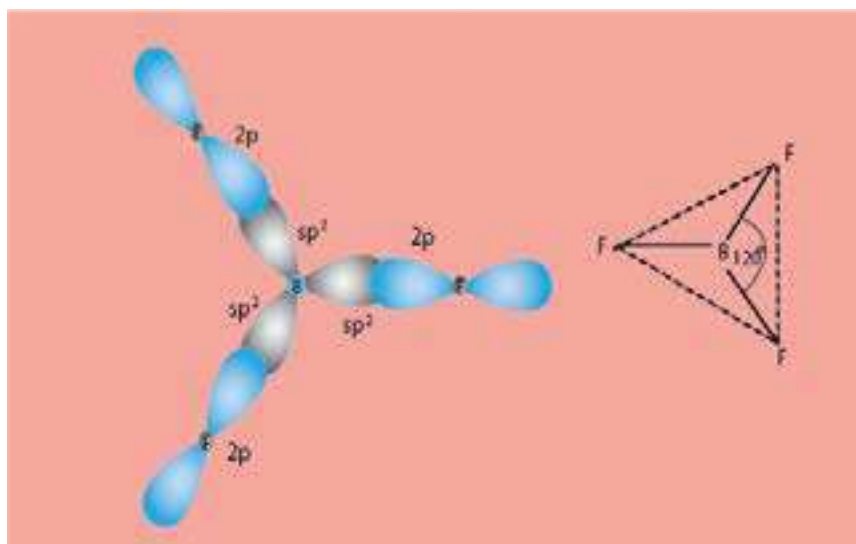
Fig. (6.15) sp^2 -p overlaps in \text{BF}_3 to form triangular planar structure.
