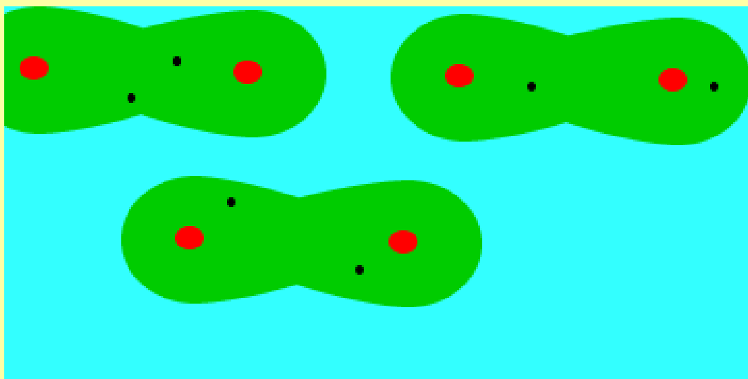
Animation 4.3 : London Dispersion Forces Source & Credit: dynamicscience
