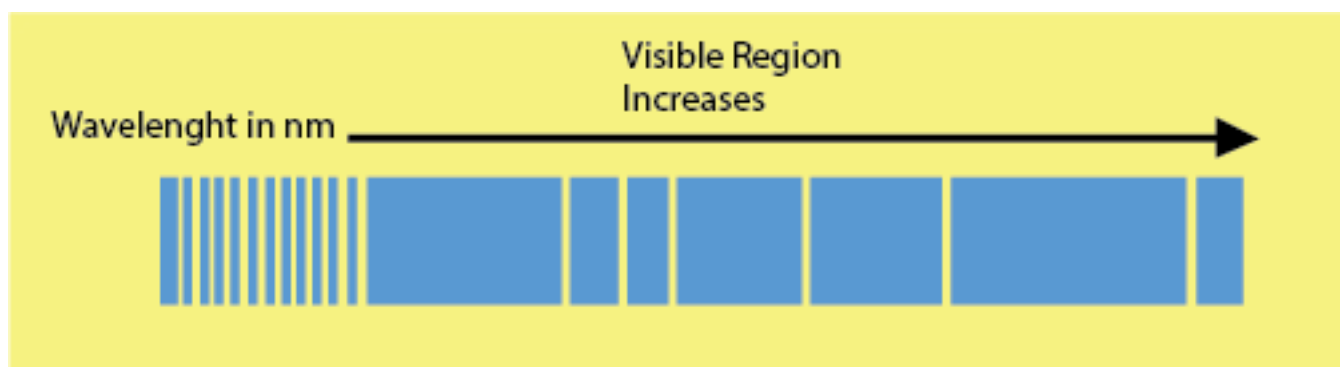
Fig (5.14) Atomic spectrum of hydrogen
