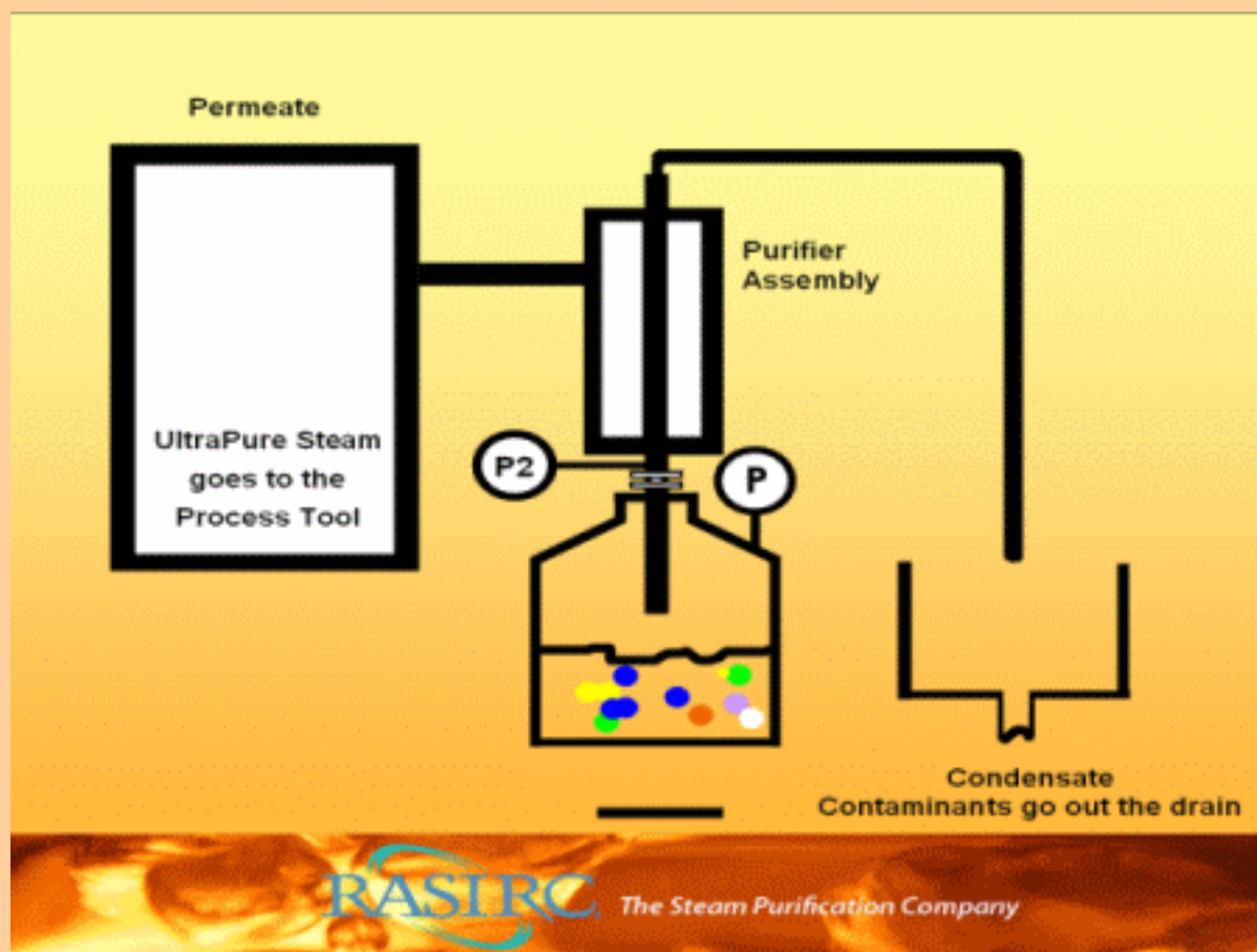
Animation 9.13: RAOULT'S LAW Source & Credit: rasirc
