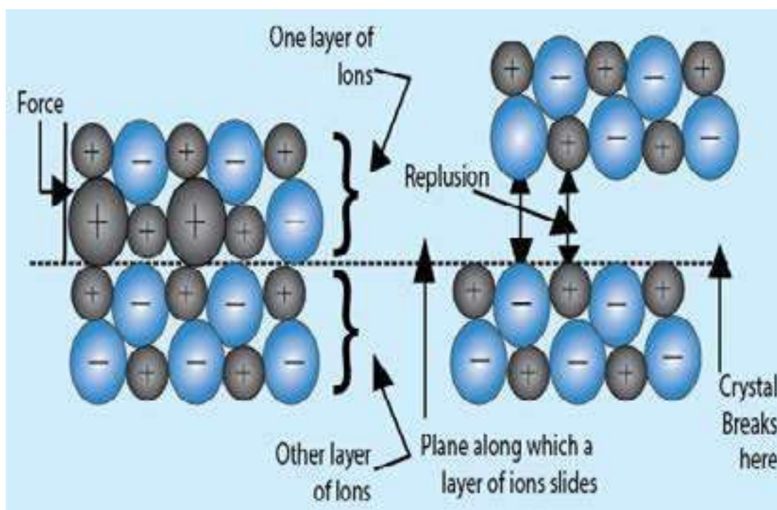
Fig (4.16) Explanation of brittleness of ionic crystals
