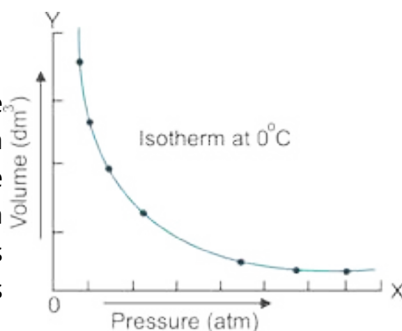
Fig (3.2) Isotherm of a gas at 0^\circ\text{C} .
