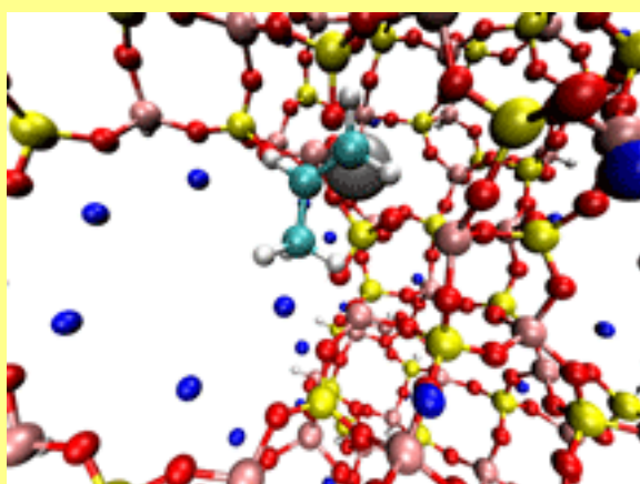
Animation 11.22: CATALYSIS Source & Credit : lsa.umich
