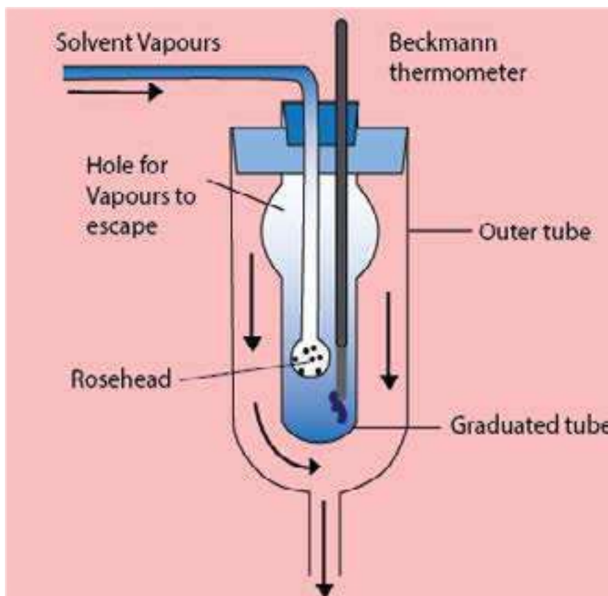
Fig (9.8) Landsberger method for measurement of elevation of boiling point
