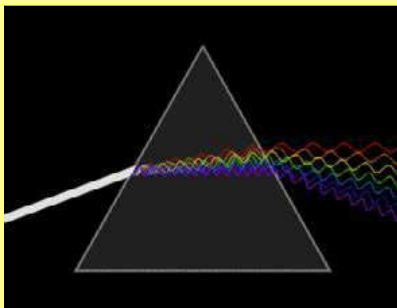
Animation 11.19: Light Source & Credit : wikipedia
