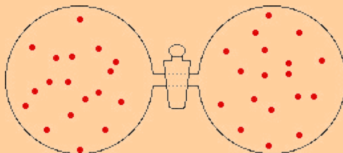
Animation 9.18: Why Some of the Properties are Called Colligative
