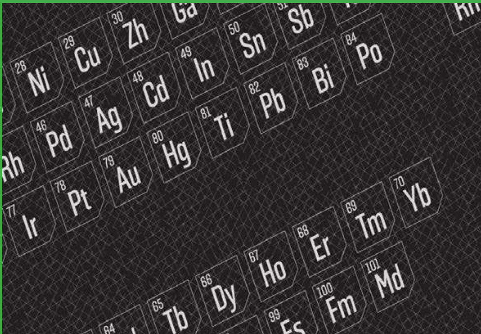
Animation 6.11: Variation of Atomic Radii in the Periodic Table Source & Credit : dynamicscience
