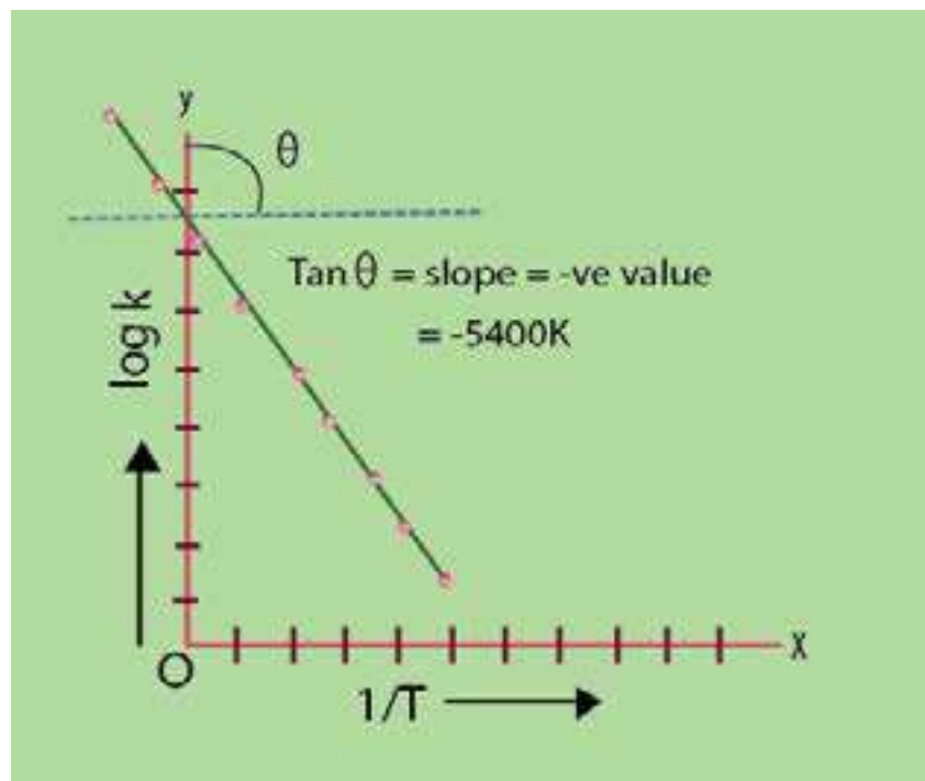
Fig. (11.8) Arrhenius plot for decomposition of \text{N}_2\text{O}_5
