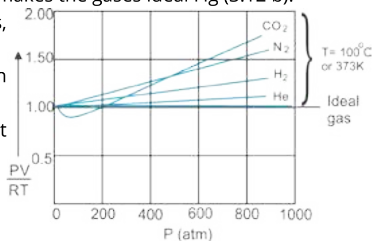
Fig (3.12 b) Non-ideal behaviour of gases at 100^\circ\text{C} .
