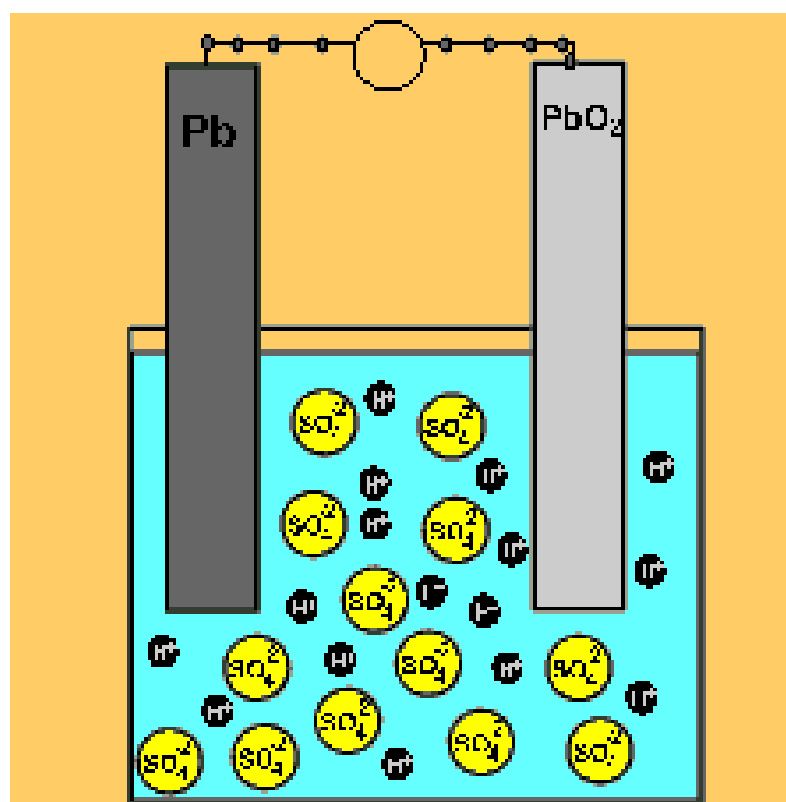
Animation 10.1: ELECTROCHEMICAL CELLS Source & Credit: dynamicscience
