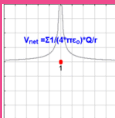
Animation 10.11: Electric potential Source & Credit : wikipedia
