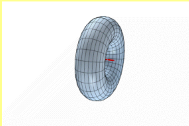
Animation 11.18: Surface Area Source & Credit : darelhardy
