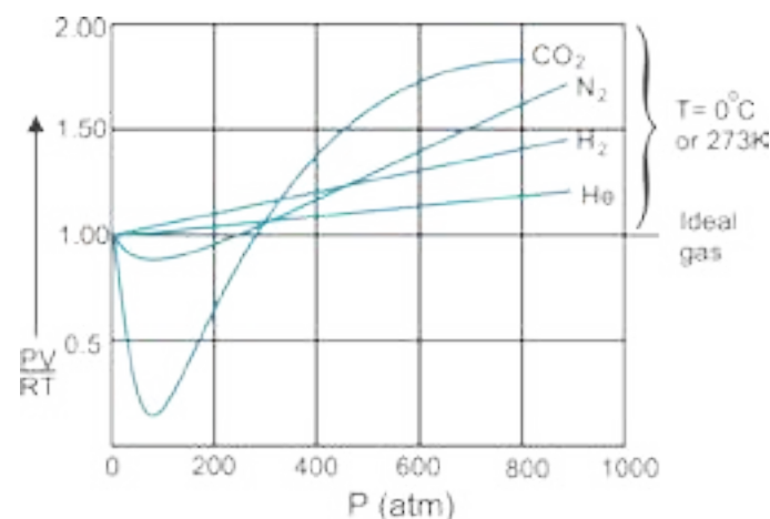
Fig (3.12 a) Non-ideal behaviour of gases at 0^\circ\text{C}
