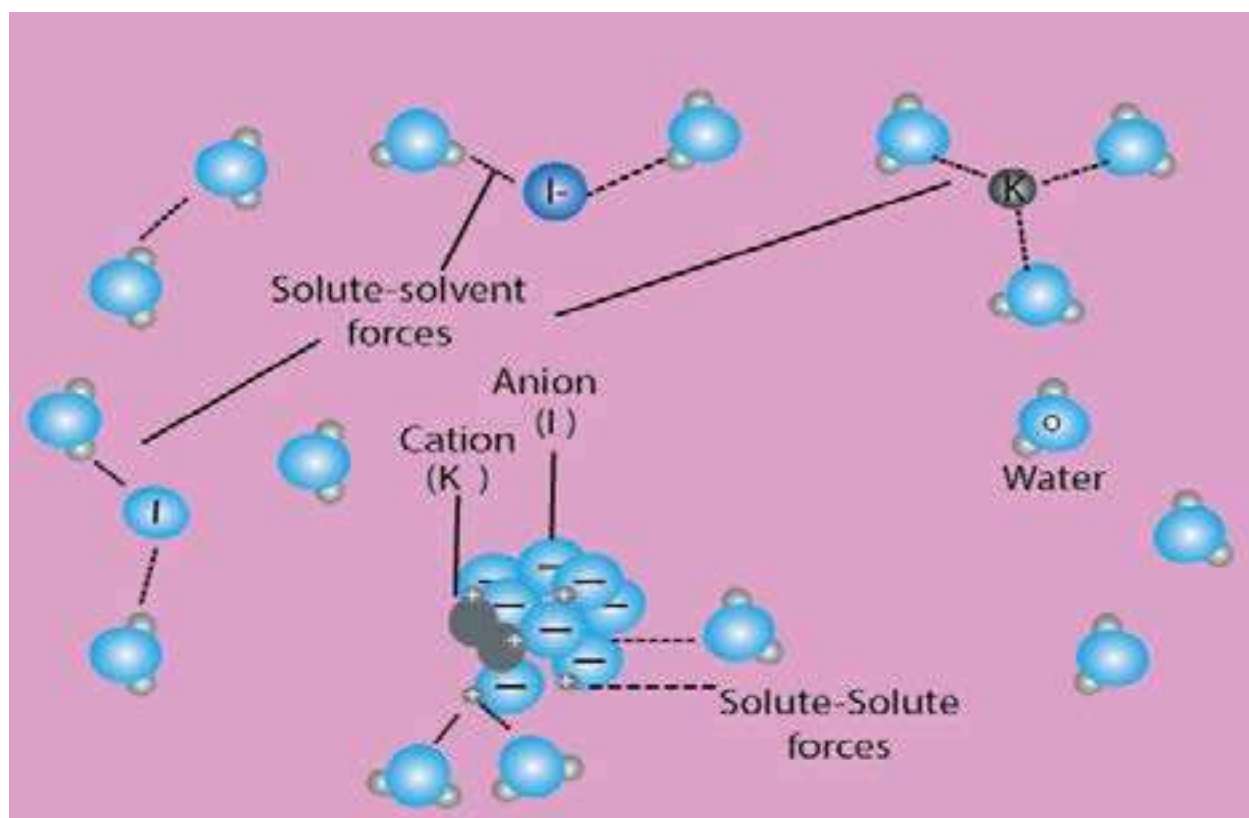
Fig (9.11) Interaction between water molecules and cations and anions provide the energy- necessary to overcome both the intermolecular forces between water molecules and the ionic bond in a potassium iodide
