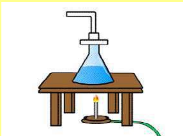
Animation 11.13: Determination of Order of a Reaction Source & Credit : askiitians
