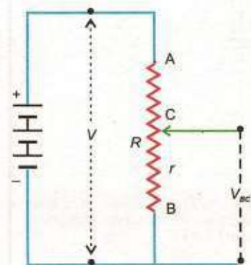
Use of rheostat as potential divider
