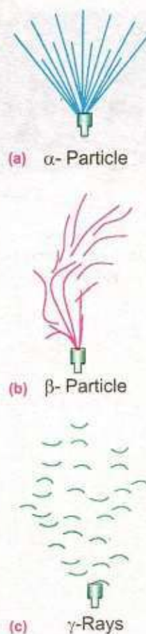
Fig. 21.8 Cloud chamber tracks of \alpha , \beta , \gamma radiations
