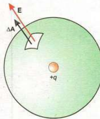
Fig. 12.14 The total electric flux through the surface of the sphere due to a charge q at its centre is q/\epsilon_0 .
