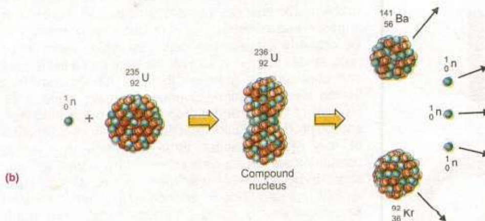
Process of Fission reaction
