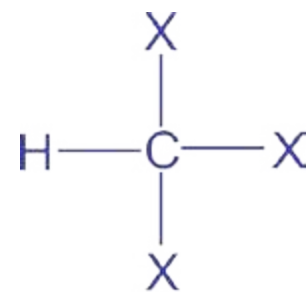
Trihaloalkane
