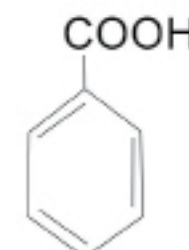
Benzoic acid
