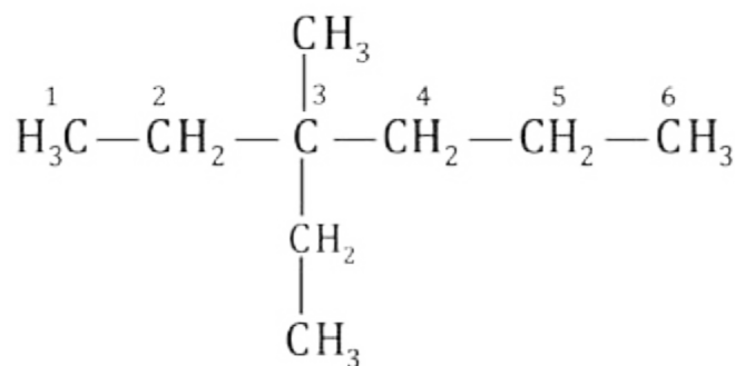
3-Ethyl-3-methylhexane
