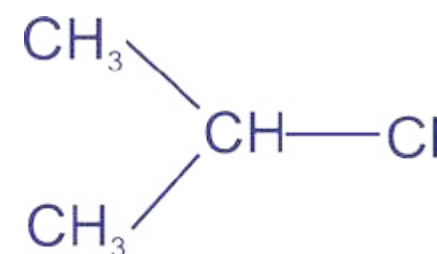
2-Chloropropane
