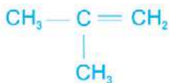
2-Methylpropene (Isobutylene)
