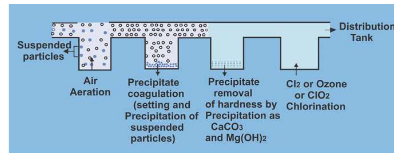
Fig. 16.1 Purification of Water
