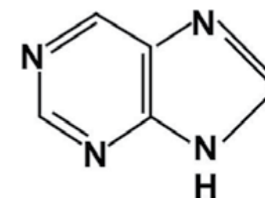
Purine
