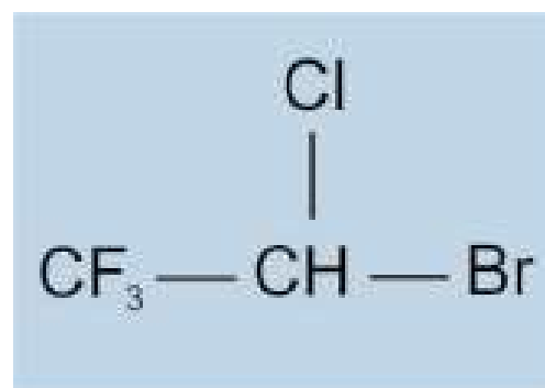
Halothane
