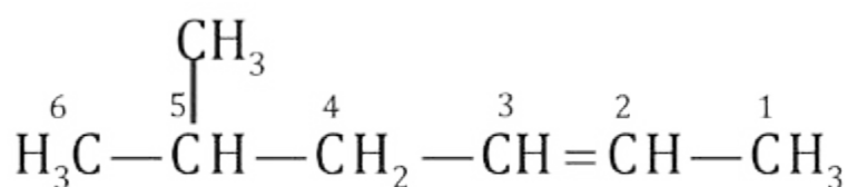
5-Methyl-2-hexene
